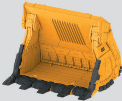
Front shovel buckets
